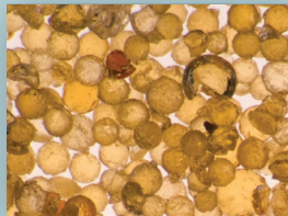
Cation Resin exposed to Chlorine (5 years later)
